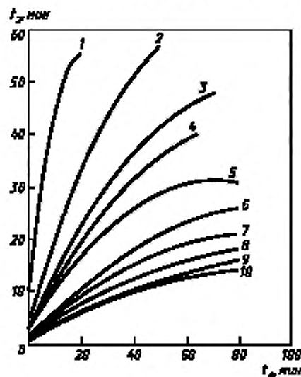
1 — H/\sqrt{F} = 1,2 ; 2 — H/\sqrt{F} = 2,0 ; 3 — H/\sqrt{F} = 2,4 ; 4 — H/\sqrt{F} = 2,85 ; 5 — H/\sqrt{F} = 3,2 ; 6 — H/\sqrt{F} = 4,0 ; 7 — H/\sqrt{F} = 4,4 ; 8 — H/\sqrt{F} = 5,2 ; 9 — H/\sqrt{F} = 5,6 ; 10 — H/\sqrt{F} = 6,0
